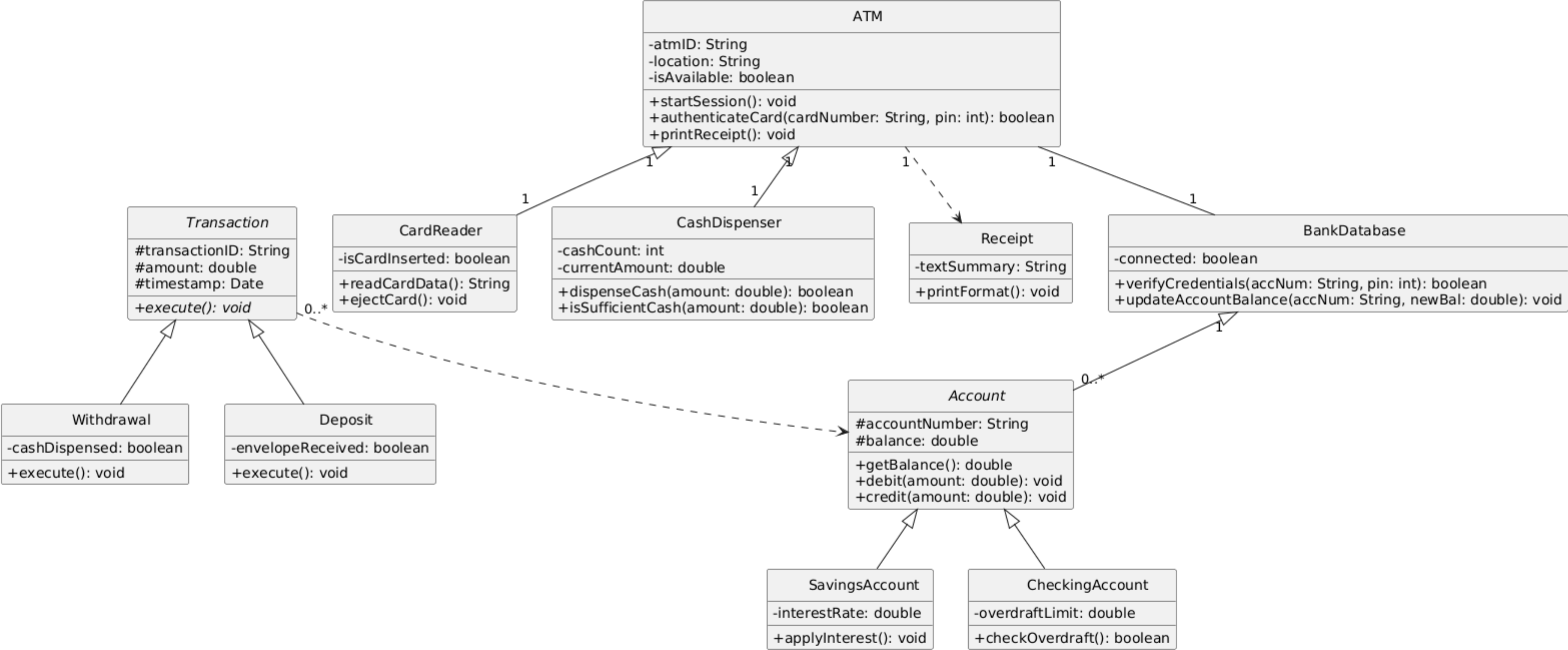
ATM System - Class Diagram
